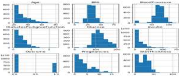
Figure4 Histogram
