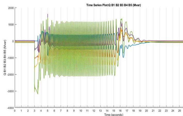
Reactive power | transient t = 21 - 3 = 18 sec
