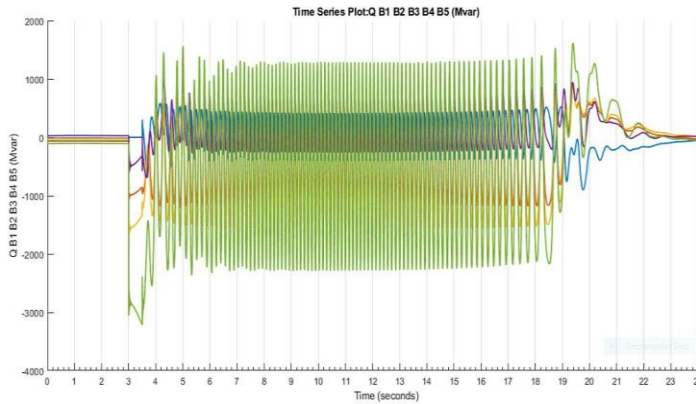
Reactive power | transient t = 24-3 = 21 sec
