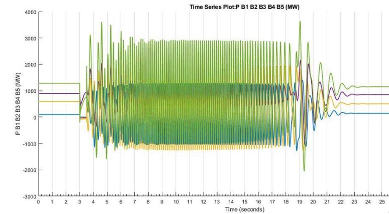
Power | transient t = 24 - 3 = 21 sec
