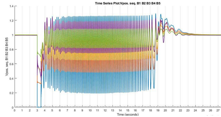
Voltage | transient t = 25 - 3 = 22 sec
