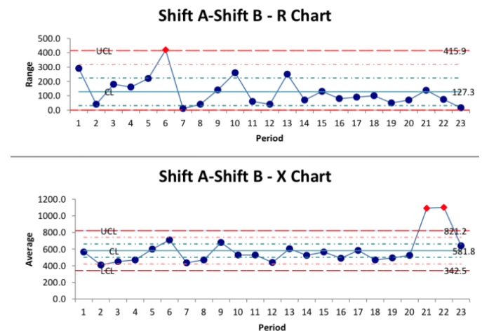
Fig. 5: Control Chart for Manufacturing Defects
