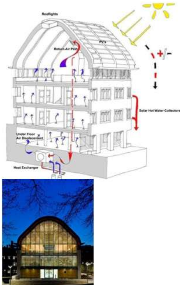
Fig. 16. Ventilation Systems
