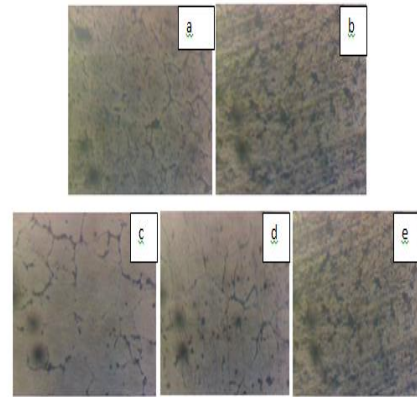
Fig Optical microstructure of (a) A7075+ 1 wt.% Graphite, (b) A7075+1 wt.% Graphite+ 0.5 wt.% Sic (c) A7075+1 wt.% Graphite+ 1 wt.% Sic (d) A7075+1 wt.% Graphite+ 1.5 wt.% Sic and (e) A7075+1 wt.% Graphite+ 2 wt.% Sic
