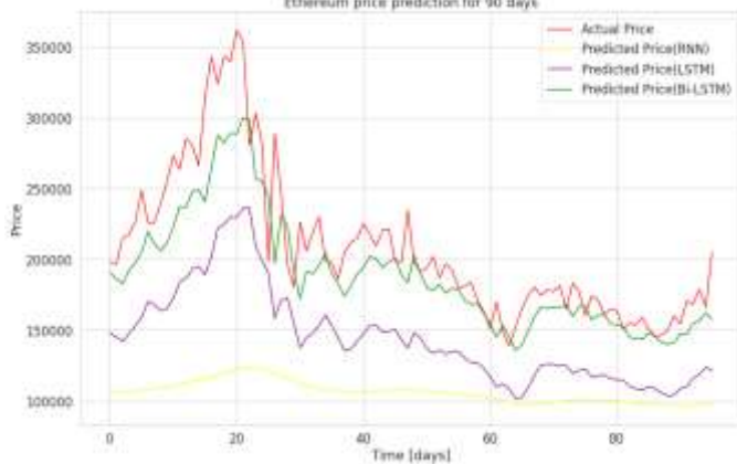
Fig. 4: 90-day price prediction
