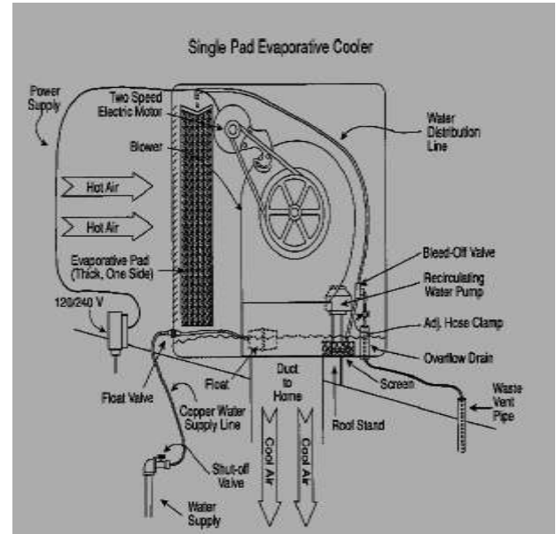
Fig. 4 Single pad evaporative cooler
