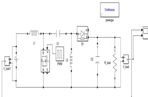
Fig. 9. SEPIC Converter
