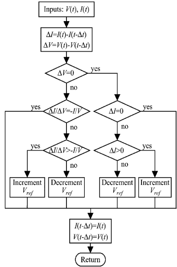
Fig. 8. Flowchart of Incremental Conductance MPPT algorithm
