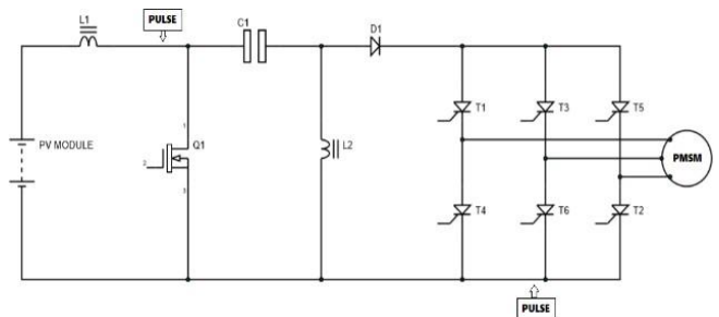
Fig. 4. Circuit Diagram
