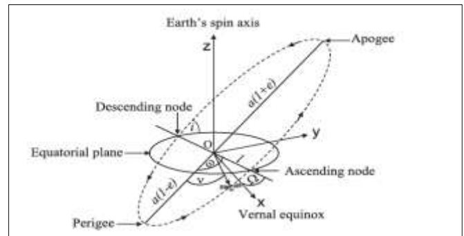
Fig.1 Graphical layout of the elliptical orbit and definition of Keplerian orbital elements [4].
