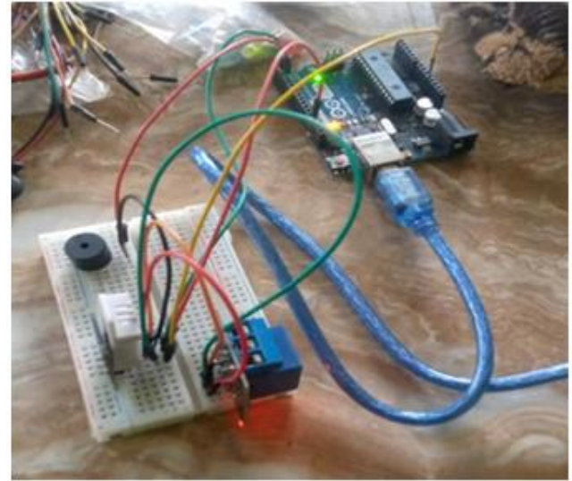
Fig. 3. Physical connection of the system
