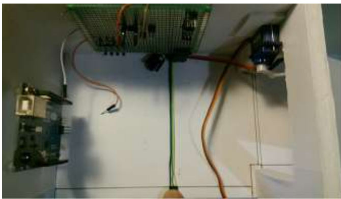
Figure 4: The microcontroller's placement
