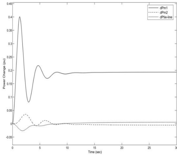
Figure 10: power deviations for ARFLFC controller.
