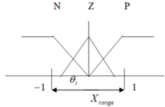
Figure 6: The membership functions used for the ARFLFC inputs variables [34]
