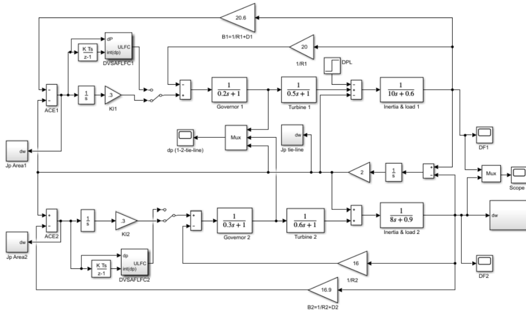
Figure2: Transfer function block diagram of two area power
