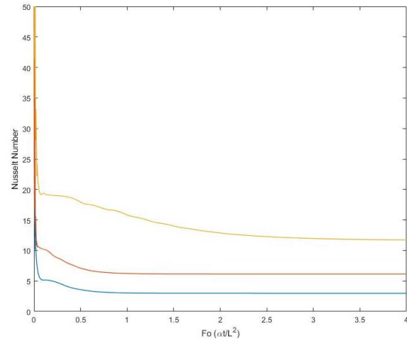
Figure 17: Nusselt number at the left boundary with Fourier number (Fo)
