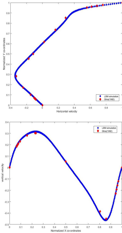
Figure 3: Plot of Horizontal and Vertical velocity with normalized co-ordinates for Re=400
