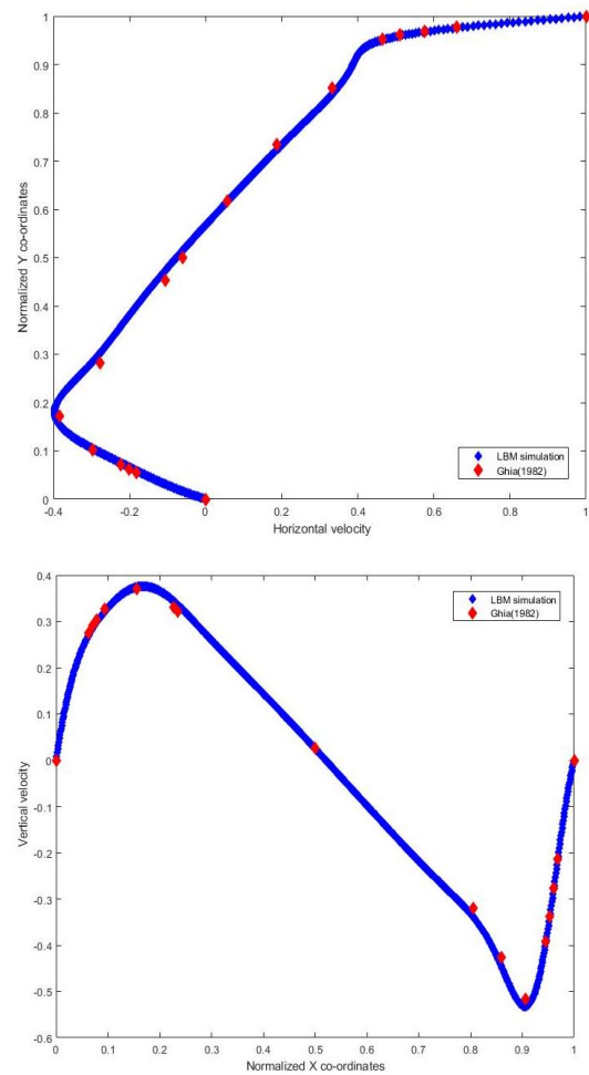
Figure 5: Plot of Horizontal and Vertical velocity with normalized co-ordinates for Re=1000
