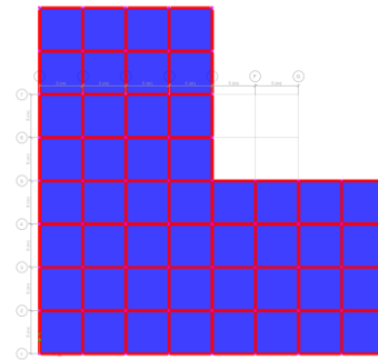
Fig 4: ETABS Plan of Conventional Slab System.
