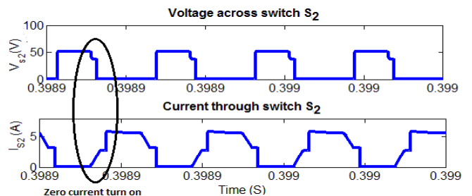
Fig .9. Zero current turn on of switch S_2
