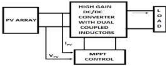
Fig. 1. PV Powered high gain DC/DC converter
