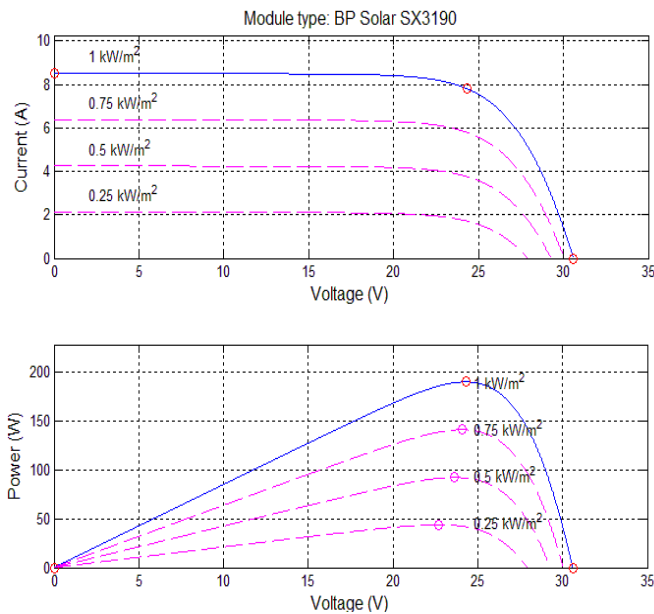
Fig .11. Characteristics of BP Solar SX3190.
