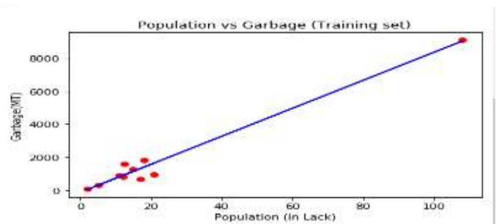
Figure 4.15: Training Set It also predicts the amount of waste generated in future using machine learning approach by taking data on cloud.
