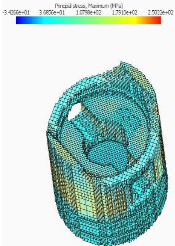
Fig 7.3 Principle maximum stress
