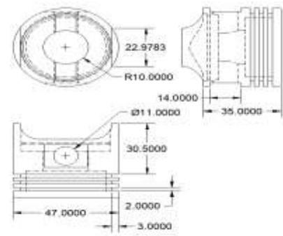
Fig 4.1 Modelling of Piston in AutoCAD
