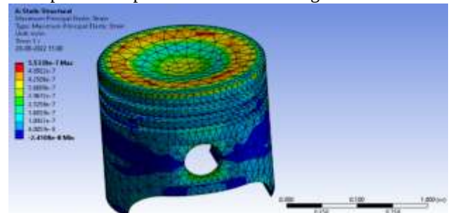
Fig 8.2.1(a) Cast Iron under Maximum principal elastic strain
