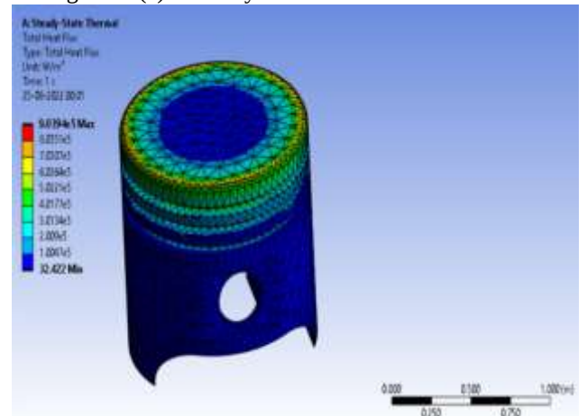
Fig 8.2.2 (f) Al Alloy under Total Heat Flux
