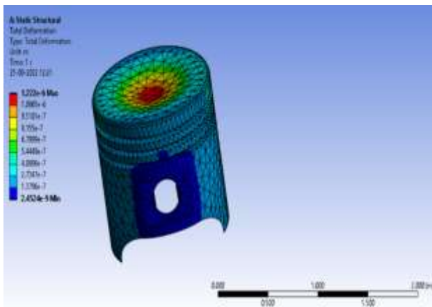
Fig 8.2.3 (b) AlSi10Mg Alloy Total Deformation
