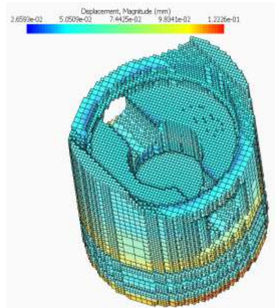
Fig 7.1 Displacement Analysis
