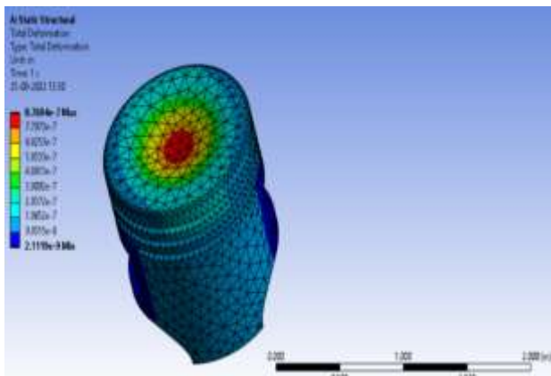
Fig 8.2.1 (b) Cast Iron under Total Deformation
