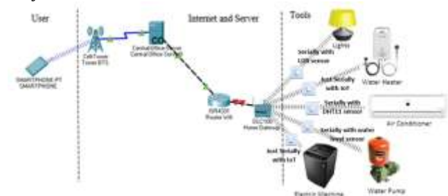
Fig. 4. Arcitekture of Systems
