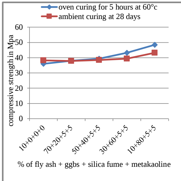
Fig. 2. % of fly ash+ggbbs+micro silica + metakaoline Vs Compressive strength of oven and ambient curing
