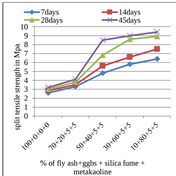
Fig. 3. % of fly ash+ggbbs+micro silica + metakaoline Vs split tensile strength
