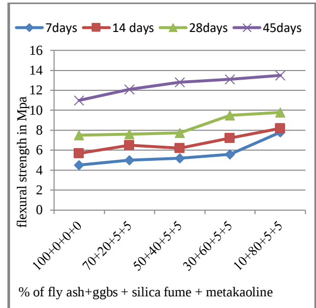
Fig 4. % of (fly ash+ggbbs+micro silica + metakaoline) Vs Flexural strength
