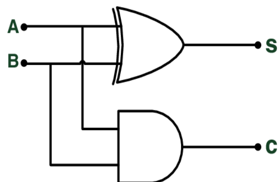
Circuit diagram of Half adder
