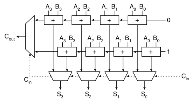
Block diagram of 4-bit Carry select adder
