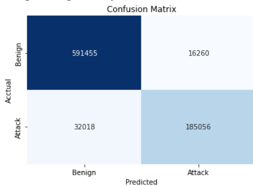
Figure 4. Confusion Matrix of Logistic Regression Classifier
