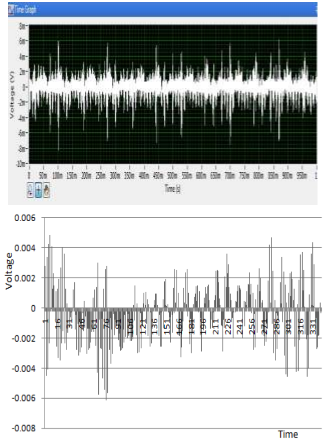
Fig 5.5 Vibration waveforms in Healthy motor condition
