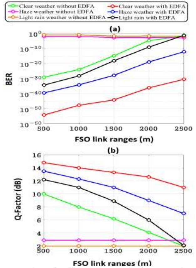
Fig. 9. Shows the effect of EDFA under diverse weather (a) BER vs. FSO link ranges (b) Q-Factor vs. FSO link ranges
