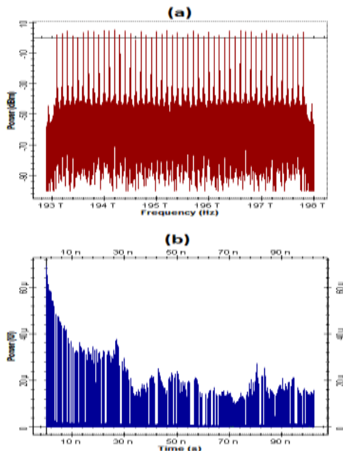
Fig. 2. Shows the emission spectrum of 48 channels (a) Transmission spectrum (b) 480 GB/s encoded data
