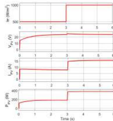
Fig. 8. Simulation results of FOC Voltage method
