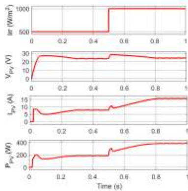
Fig. 10. Simulation results of P & O method
