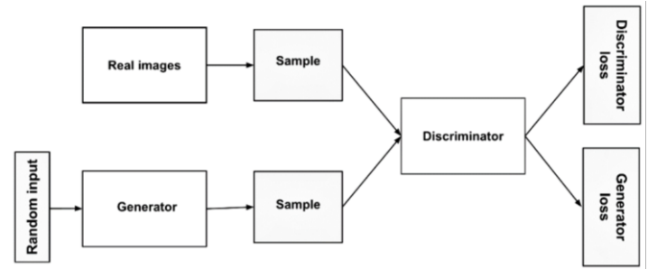
Fig. 4. GAN architecture
