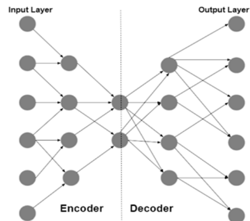
Fig. 5. Autoencoder architecture
