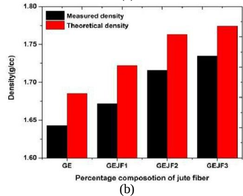
Fig.11: (a). The variation of impact strength versus composition of jute fiber; (b) The variation of densities of laminates composites
