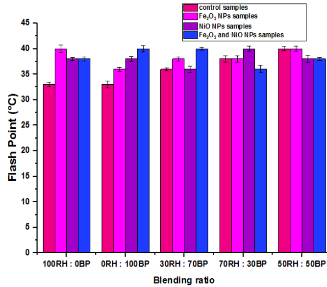
Fig 7: Flash points of bioethanol produced under different treatments with nanoparticles
