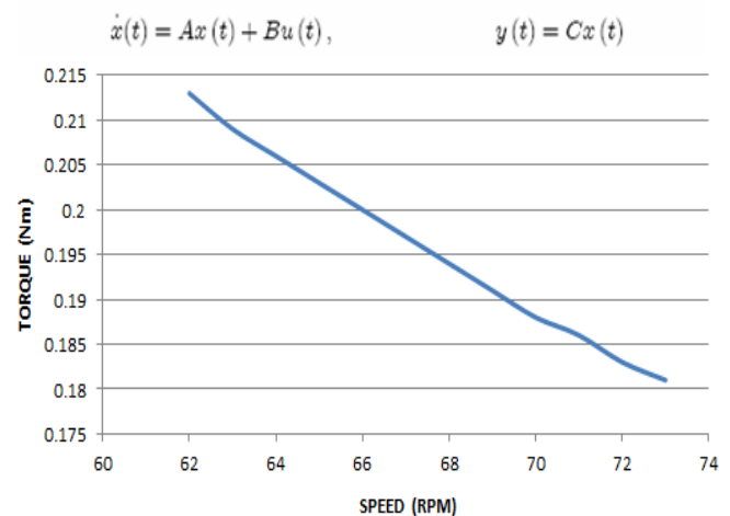
Fig.6. Speed vs. Torque Characteristics
