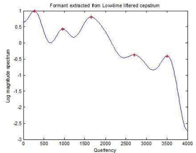
Fig. 6. Low time liftered cepstrum of Sp4 for word "Authorize".
