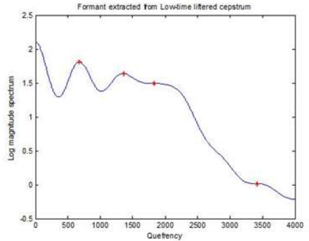
Fig. 5. Low time liftered cepstrum of Sp3 for word "Authorize".
