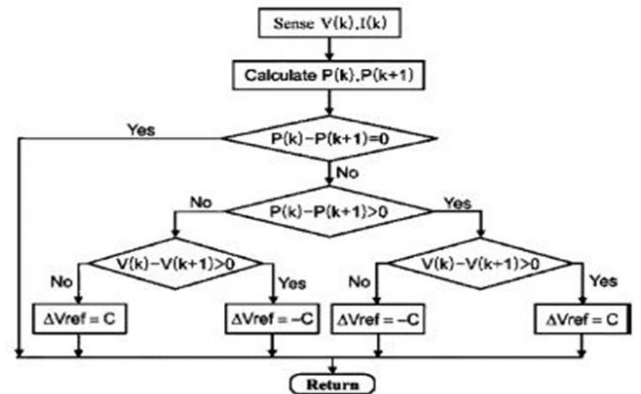
Figure 3: P & O algorithm
