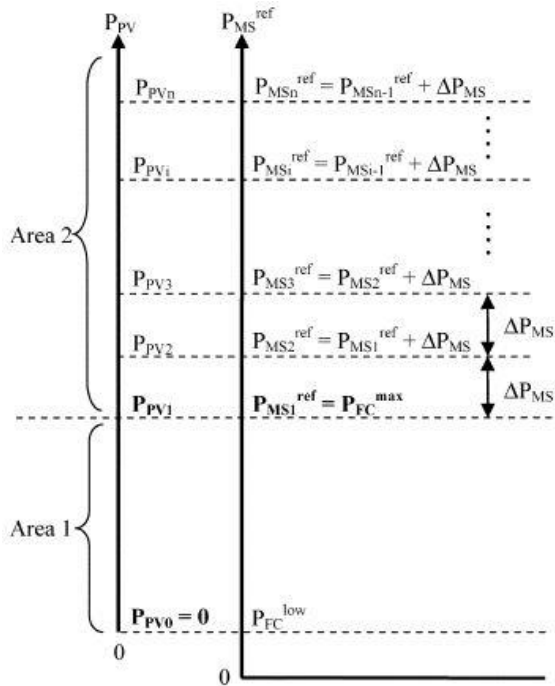
Figure 5: Operation Strategy of hybrid source in the UPC mode.
