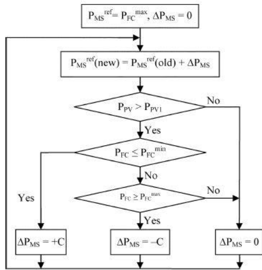
Figure 6: Control algorithm diagrams in the UPC mode ( P_{MS}^{ref} automatically changing)
