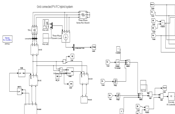
Figure 11: operating strategy of the hybrid system using hysteresis
