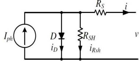
Figure 2: Equivalent representation of a PV panel
