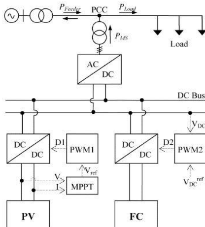
Figure 1: Grid-Connected PV-FC hybrid system.
