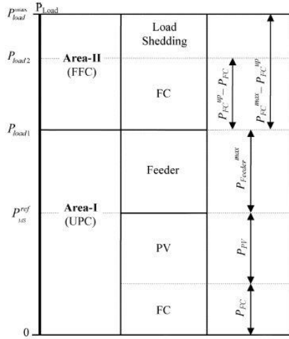
Figure 8: overall operating strategy of a grid connected Hybrid System
