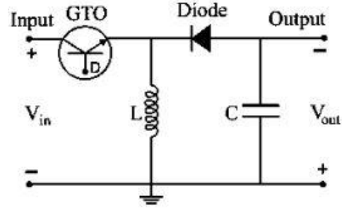
Figure 4: Buck-Boost topology
