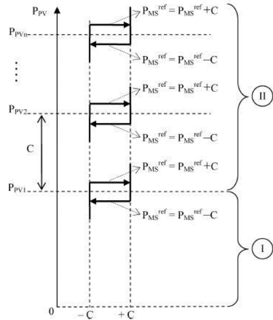
Figure 7: Hysteresis control scheme for P_{MS}^{ref} control
