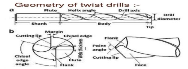
Fig 1.1 Nomenclature of Drill bit
