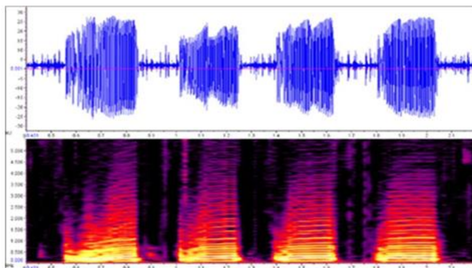
Fig 2.1: Signal Pre-processing
