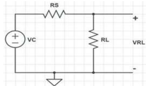
Fig. 7. Equivalent circuit diagram of the MQ-135 gas sensor
