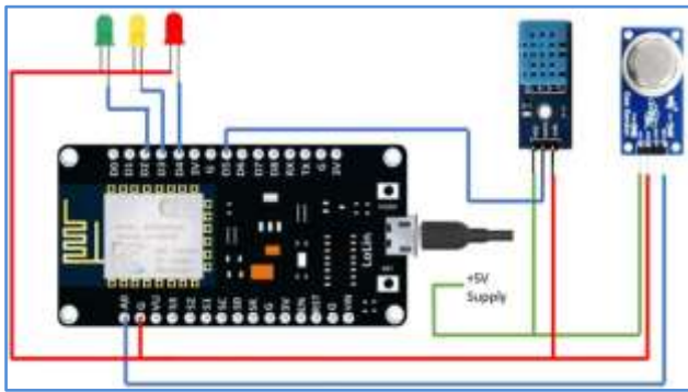
Fig. 6. Complete circuit diagram of the Setup
