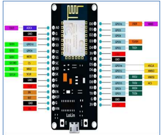
Fig. 2 The pin diagram of a NodeMCU (ver.3)
