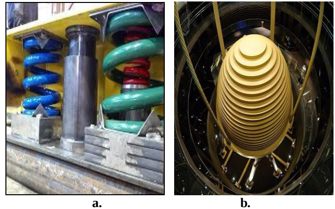
Figure 11 a. Tuned Mass Damper-Thornton Tomasetti. b. Scheme Tuned Mass Damper.
