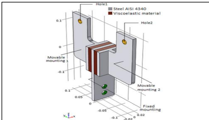
Figure 9 Viscoelastic Damper
