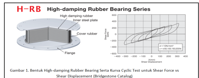
Figure 5 High-Damping Rubber.
