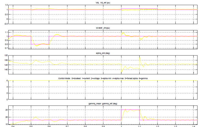
Fig 5. Inverter DC quantities
