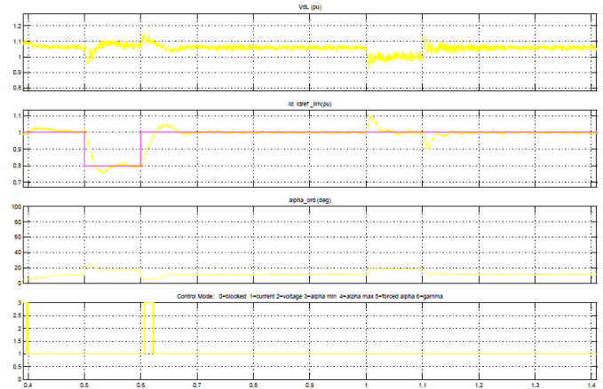
Fig 4. Rectifier DC quantities
