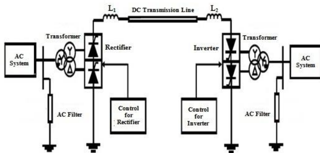
Fig 1. The monopolar HVDC transmission system model
