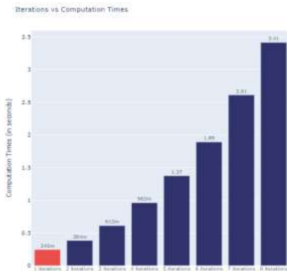
Fig 6.1: Computation of iterations with time
