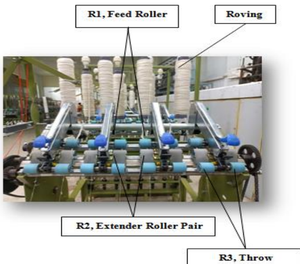
Fig.2 Feed Rollers
