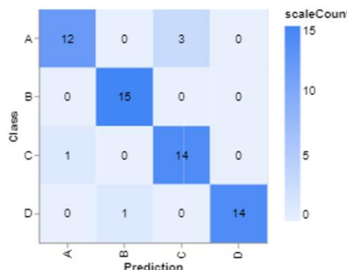
Fig. 12. Confusion Matrix
