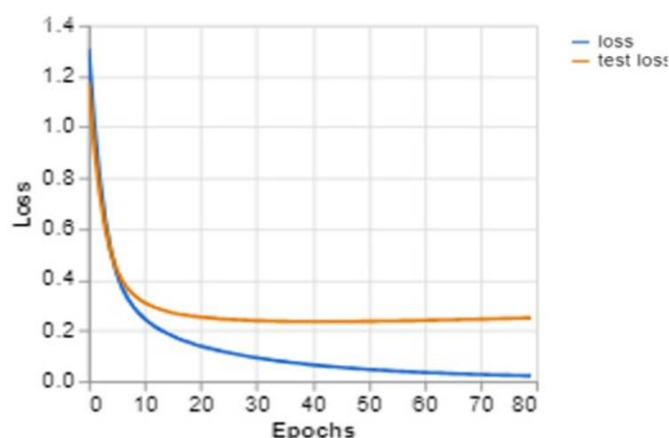
Fig. 10. Loss graph
