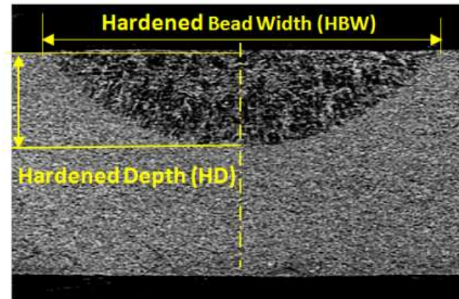
Figure. 3. Microstructure of Hardened - Bead Profile with parameters, HBW, HD and AEHB
