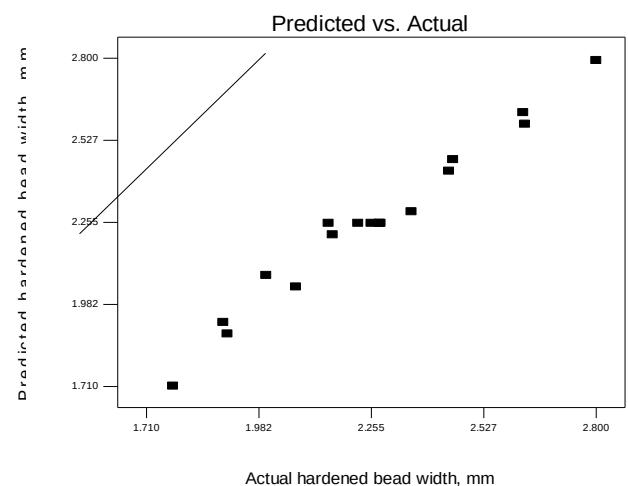
Figure 4. Scatter diagram of hardened bead width (HBW)
