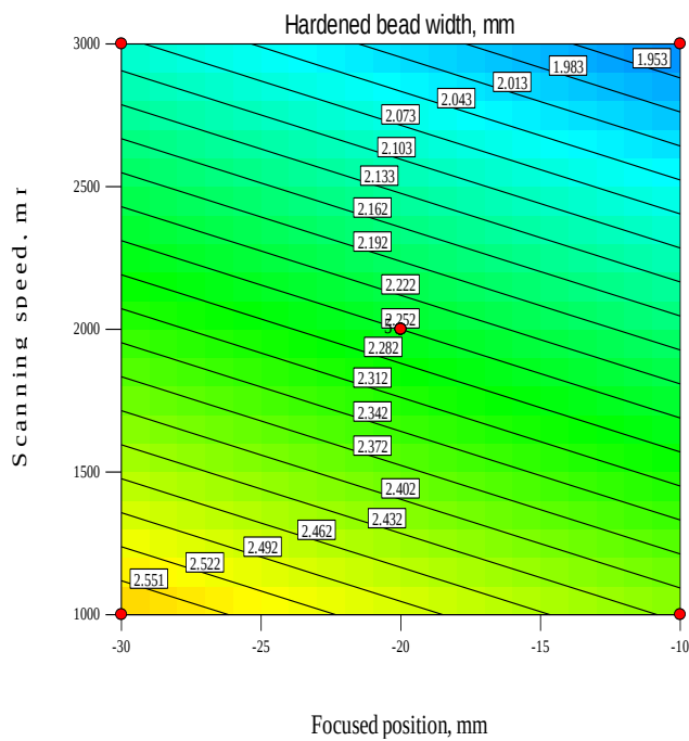
Figure 11. Contours graph shows the effect of SS and FP on the hardened bead width
