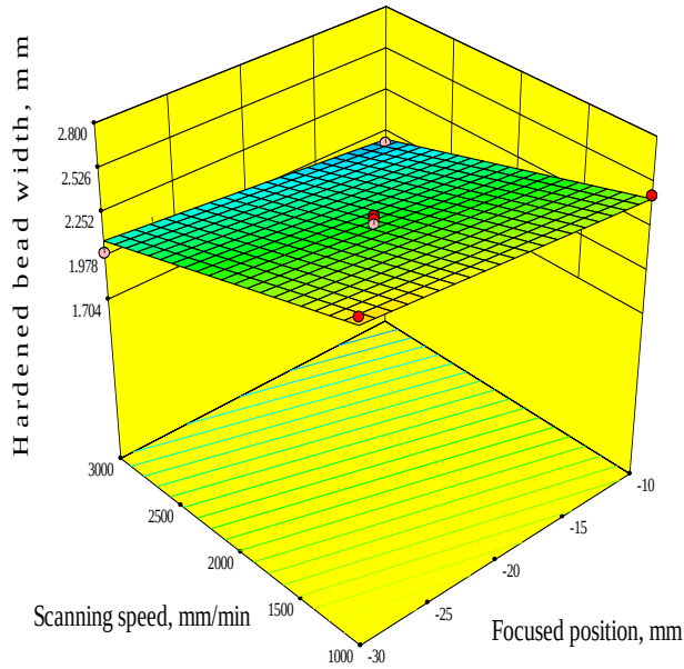
Figure 10. 3Dgraph shows the effect of SS and FP on the hardened bead width
