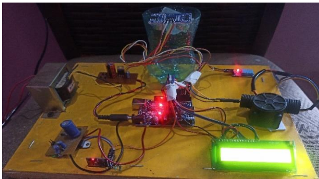
Figure 3: Hardware Implementation
