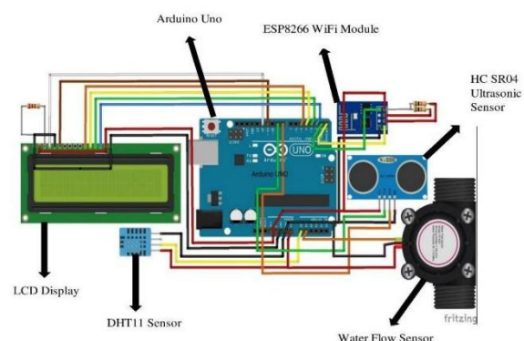
Figure 2: Circuit Diagram
