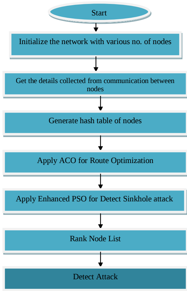
Fig 4: Proposed Methodology
