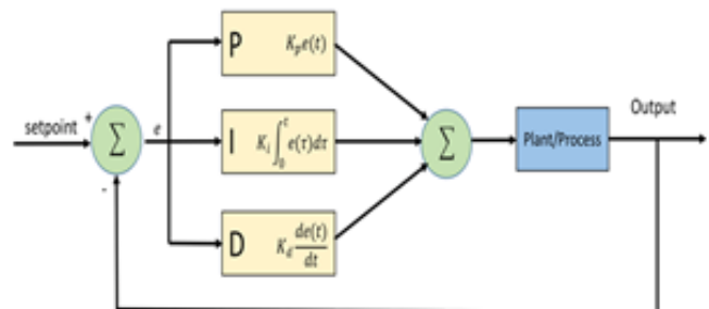
Fig. 3. PID controller with feedback
