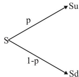
Fig 1.3(a): Binomial model for stock price
