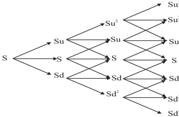
Fig1. 6 stock price with multi periods for trinomial option price
