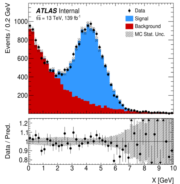
Fig.1 Basic Graph Representation of Signal and Background Events
