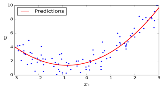
Fig 3: Simple Polynomial regression graph
