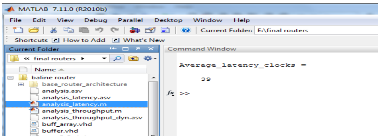
Fig. 10. Average Latency.
