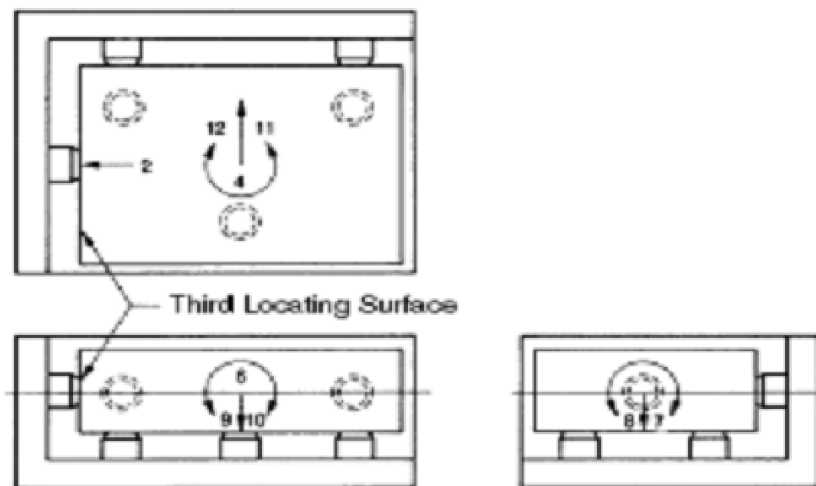
Fig 2. 3-2-1 Principle
