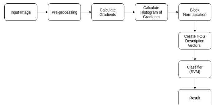
Figure: Steps for Object Detection with HOG
