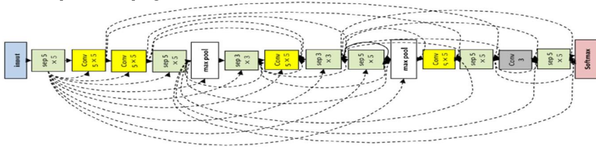
Fig 14: ENAS architecture [17]
