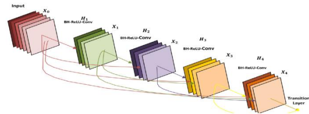
Fig 12: Architecture of DenseNet model [15]
