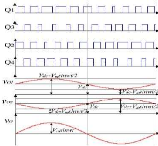
Fig. 2. Traditional modulation strategies and key waveforms
