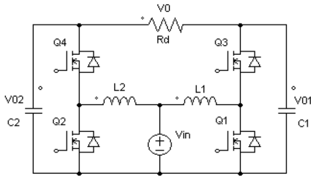
Fig. 1. Differential Boost inverter circuit diagram
