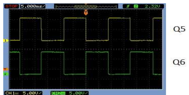
Fig. 12. Gate pulses of Switches Q5 and Q6
