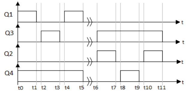
Fig. 3. Control strategy under half cycle modulation.
