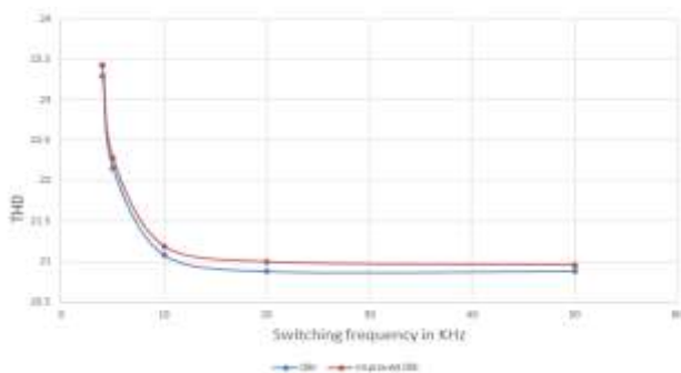
Fig. 15. Comparison between DBI and Improved DBI for Different frequencies
