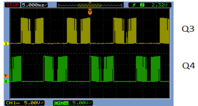
Fig. 11. Gate pulses of Switches (a) Q3 and Q4
