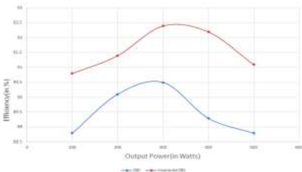
Fig. 16. Measured Efficiency of DBI and Improved DBI
