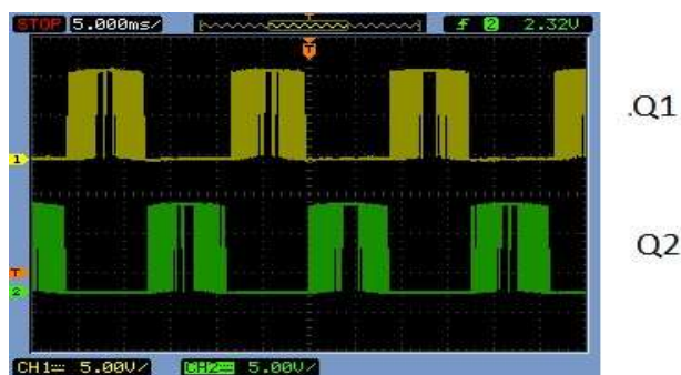
Fig. 10. Gate pulses of Switches (a) Q1 and Q2
