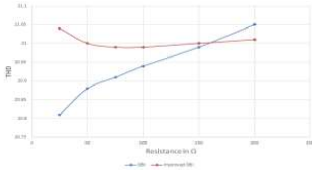
Fig. 14. Comparison between DBI and Improved DBI for Different Load Resistance
