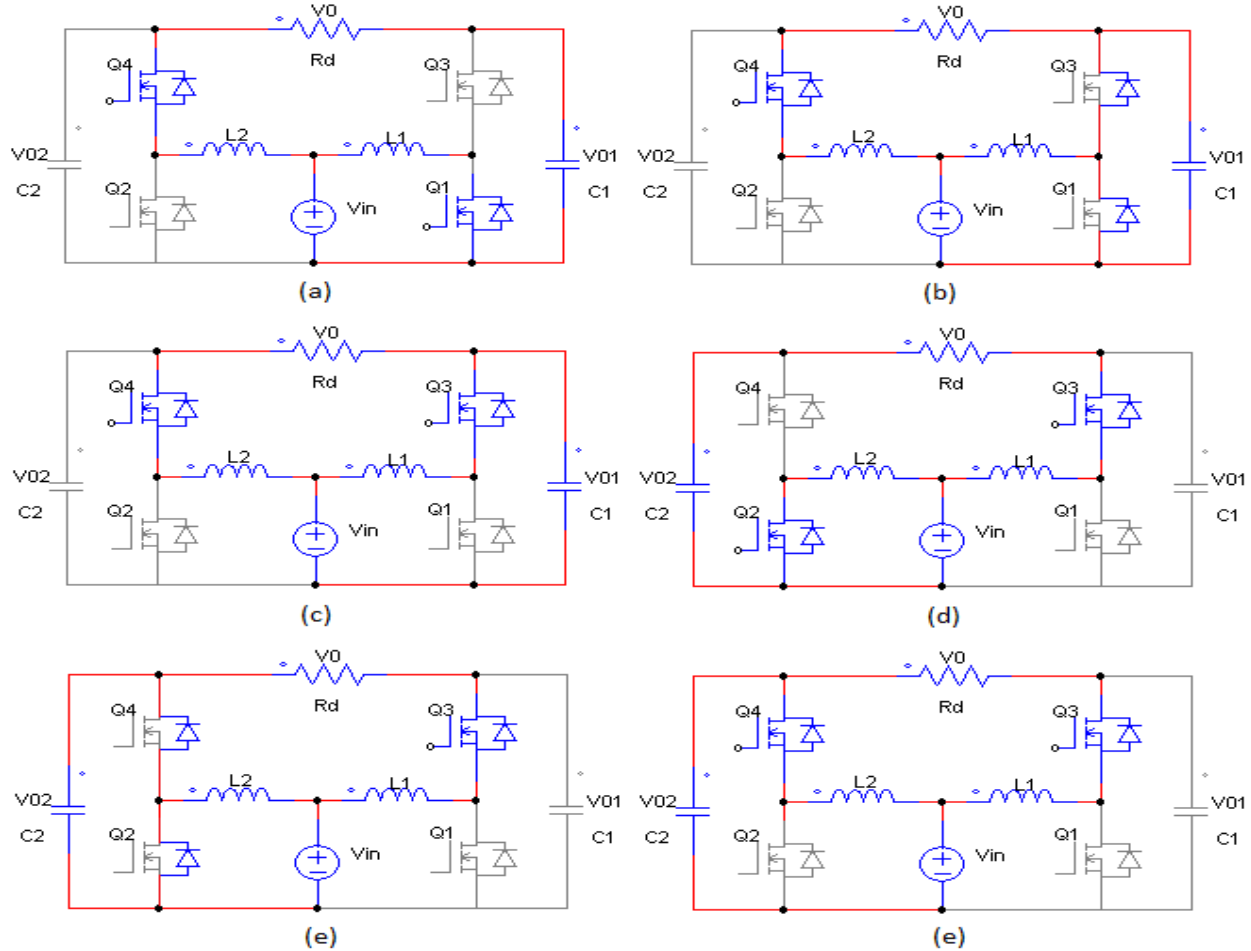
Fig. 4. Equivalent circuits of switching modes. (a) [ t_0, t_1 ], (b) [ t_1, t_2 ] or [ t_3, t_4 ], (c) [ t_2, t_3 ], (d) [ t_6, t_7 ], (e) [ t_7, t_8 ] or [ t_9, t_{10} ] and [ t_{10}, t_{11} ]
